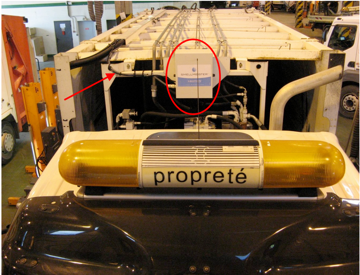
View of the diffusion ramp installed in the back of the truck:
